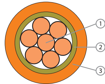
Component 1. Plain Annealed Copper Wire 2. Mica Tape 3. Cross-linked Polyolefin Low Smoke Zero Halogen Compound
